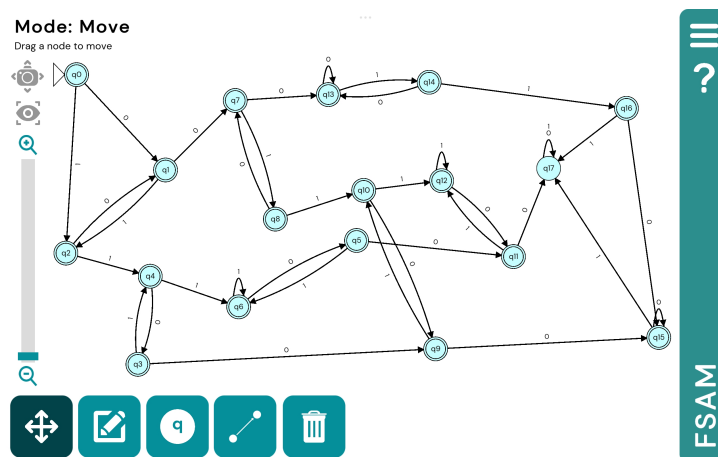
Figure 11: DFA Diagram for at least One pair of "0" or "1"
